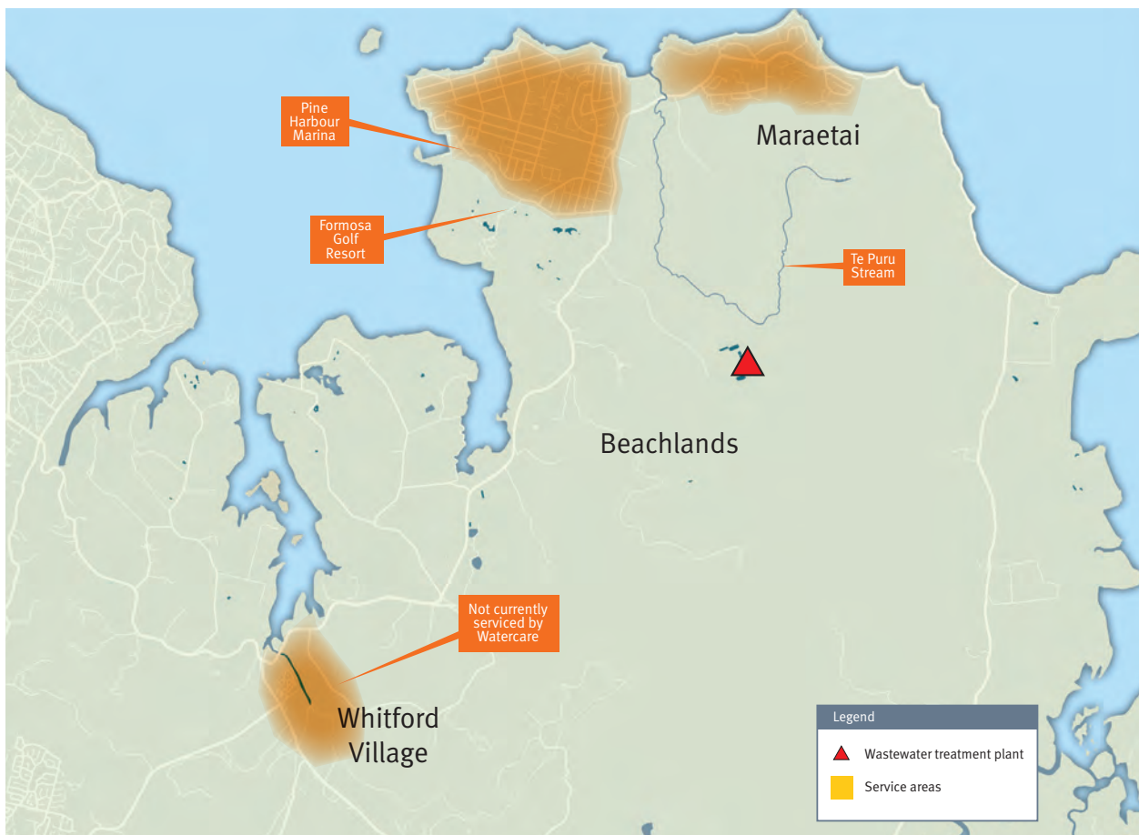
Figure 1: Beachlands-Maraetai and Whitford Village locality map
