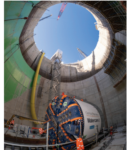
TBM at Māngere Pump Station
